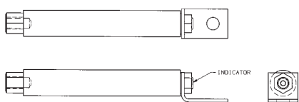
TYPE 30 - EXTERNAL FEMALE TO BOLT (L BRACKET)
